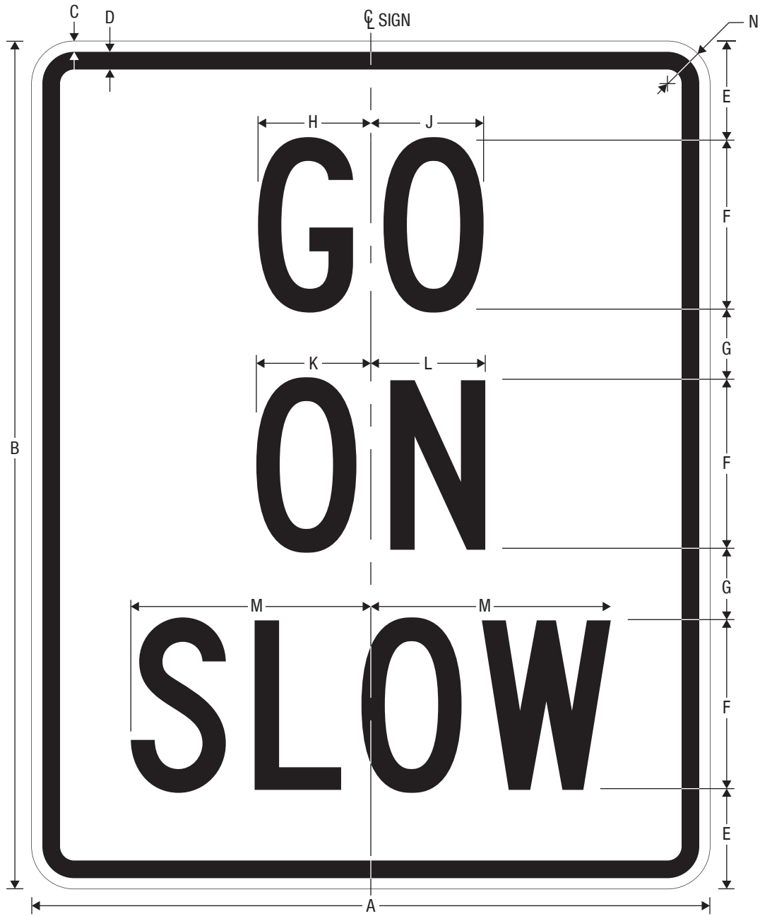
R1-8 GO ON SLOW
